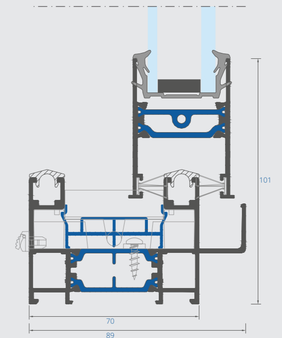
Excellence U w = 1,4
